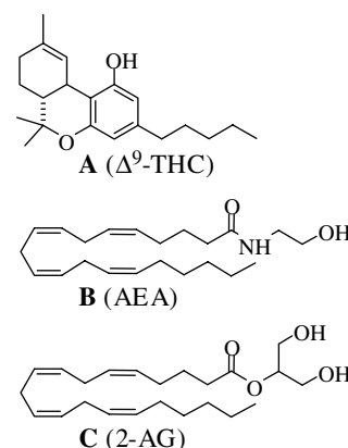
Figure 1. Cannabinoid derivatives.
