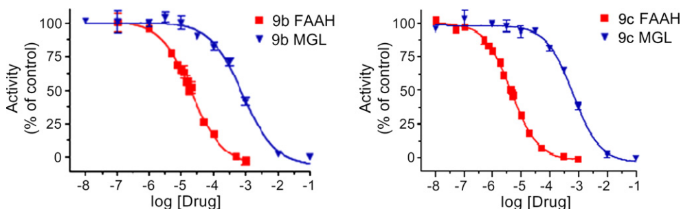
Figure 3. Azetidinone inhibitors of FAAH and MGL, 9b and 9c .
