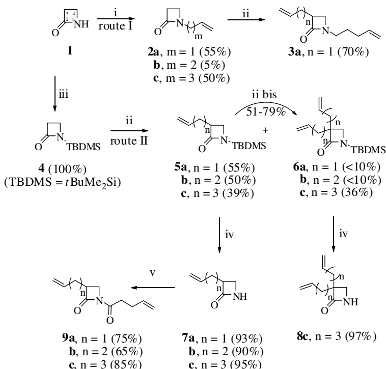
Scheme 1. Synthesis of 1,3-substituted azetidinones. Reagents and conditions: (i) alkenyl bromide, K 2 CO 3 , Bu 4 NBr catal., CH 3 CN, 80 °C, 15 h; (ii) LDA, THF, –78 °C, 0.5–1 h; then alkenyl bromide, –78 to 20 °C, 15 h; (iii) t BuMe 2 SiCl, DIEA, CH 2 Cl 2 , 20 °C, 24 h; (iv) CsF, MeOH, 20 °C, 2 h; (v) acid chloride, pyridine, CH 2 Cl 2 , 20 °C, 4 h.
